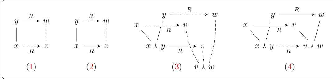
Figure 2: The four conditions of a modal L-frame. Lines denote the poset order, with high nodes being bigger. Arrows denote the relation R .
