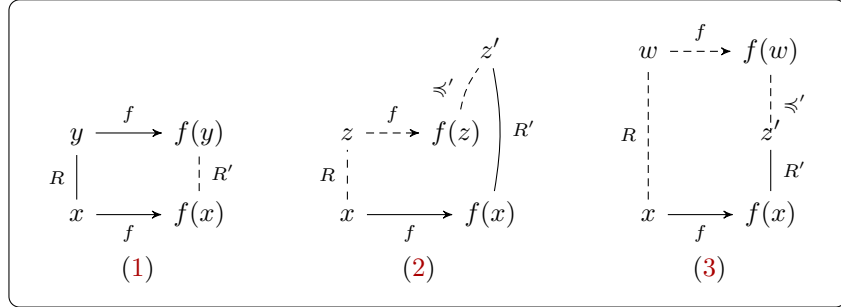
Figure 3: The conditions of a bounded L-morphism.
