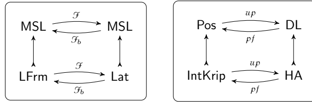
Figure 1: Functors between categories of (semi)lattices. The upper rows are dual adjunctions. up takes a poset to its lattice of upsets, and pf takes a lattice to its ordered set of prime filters.
